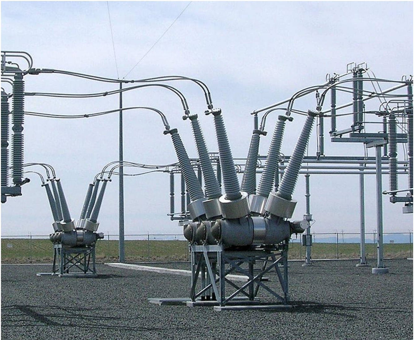
Substation Power Circuit Breaker (Example)
