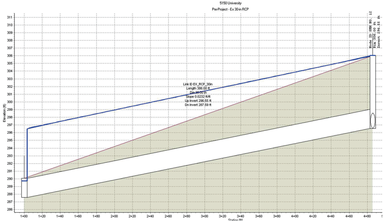
Figure 6-1: Pre-Project Hydraulic Profile (S&S Analysis)
