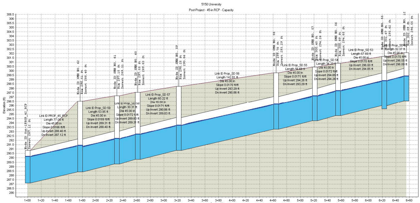
Figure 6-4: Post-Project, 48-inch RCP, Hydraulic Profile (S&S Analysis) – Capacity Analysis
