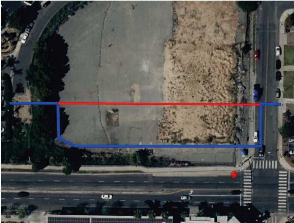
Figure 6-3: Proposed Re-alignment and upsized RCP Storm Drain (blue)
