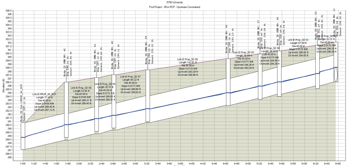
Figure 6-5: Post-Project, 45-inch RCP, Hydraulic Profile (S&S Analysis) – Upstream Limitations
