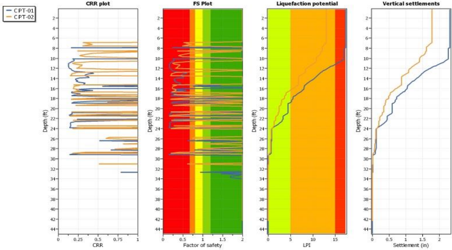
FIGURE C-1 LIQUEFACTION ANALYSIS USING IDRISSE AND BOULANGER 2014 GRANADA COMMUNITY CENTER AND BURNHAM PARK HALF MOON BAY, CALIFORNIA
