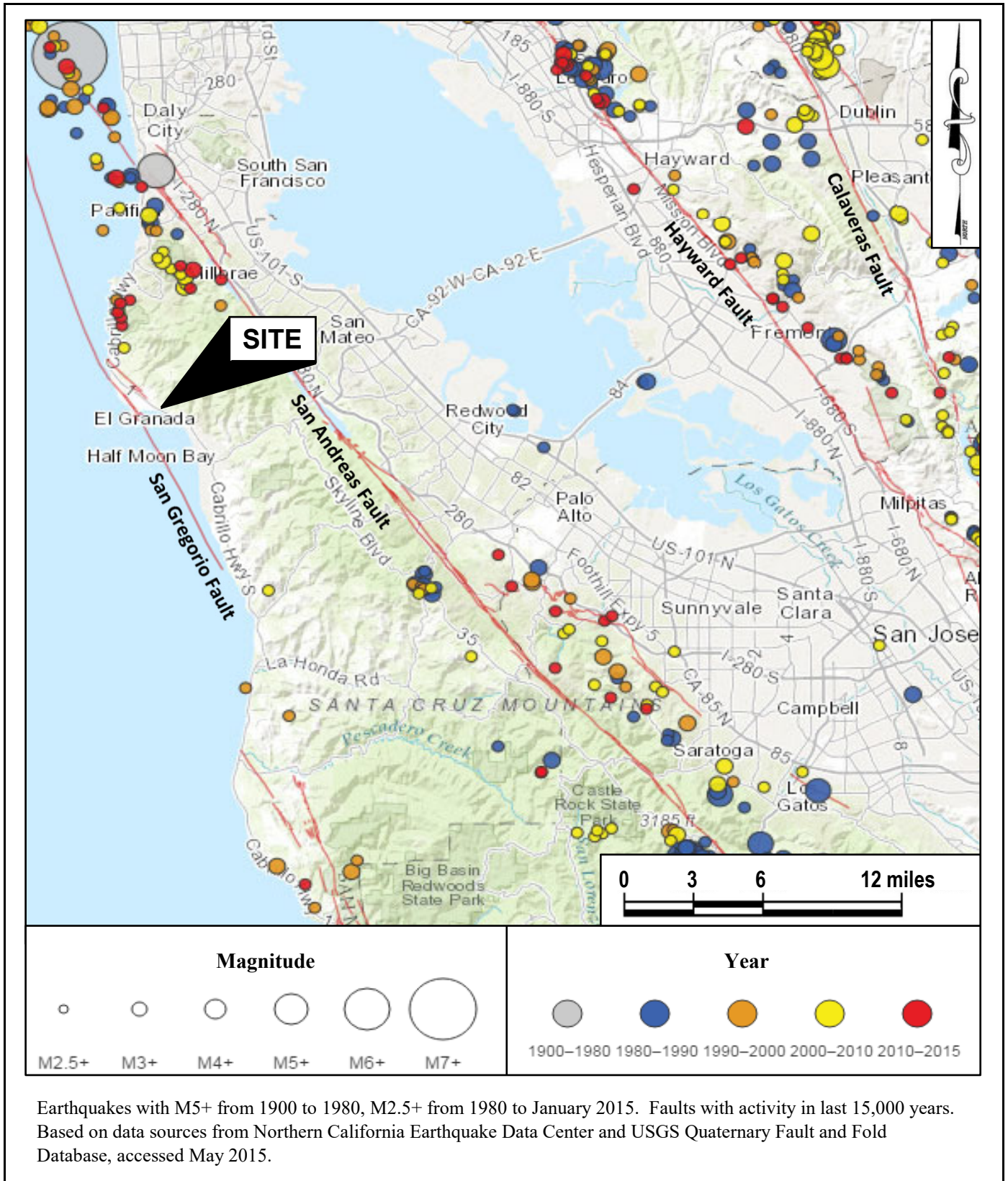
REGIONAL FAULT AND SEISMICITY MAP GRANADA COMMUNITY CENTER AND BURNHAM PARK HALF MOON BAY, CALIFORNIA
