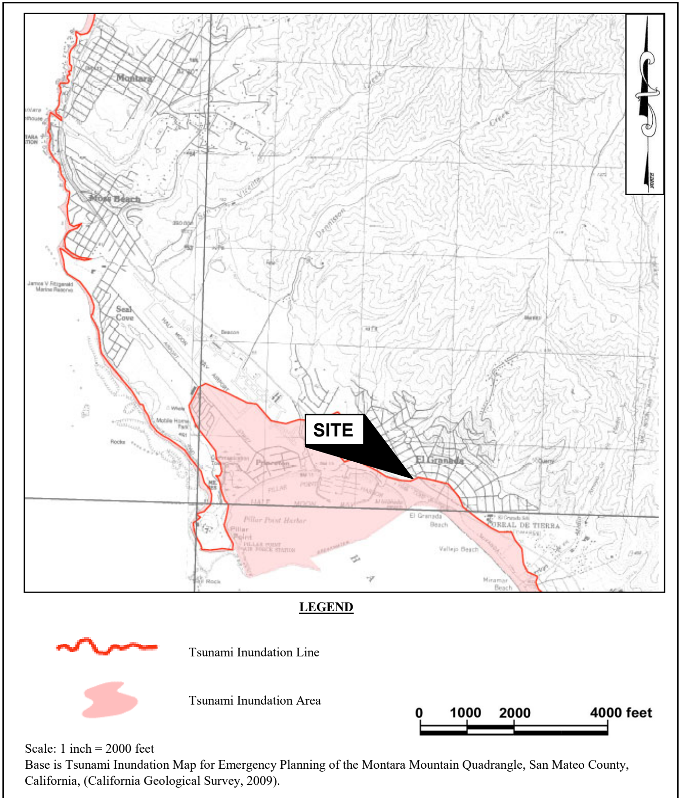
TSUNAMI INUNDATION MAP FOR EMERGENCY PLANNING GRANADA COMMUNITY CENTER AND BURNHAM PARK HALF MOON BAY, CALIFORNIA
