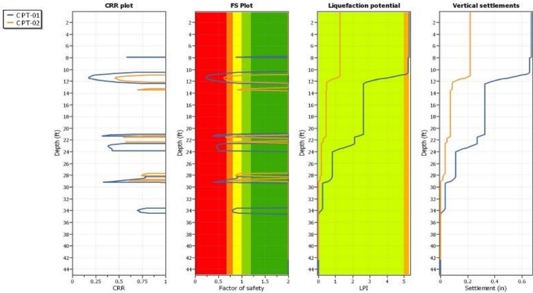
FIGURE C-2 LIQUEFACTION ANALYSIS USING ROBERTSON 2009 GRANADA COMMUNITY CENTER AND BURNHAM PARK HALF MOON BAY, CALIFORNIA
