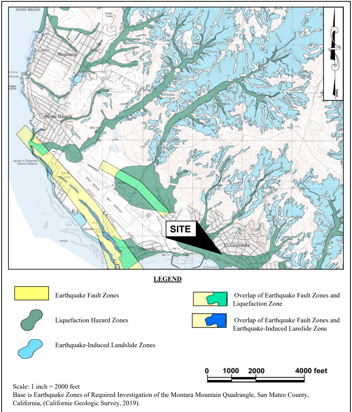
STATE SEISMIC HAZARD ZONES GRANADA COMMUNITY CENTER AND BURNHAM PARK HALF MOON BAY, CALIFORNIA
