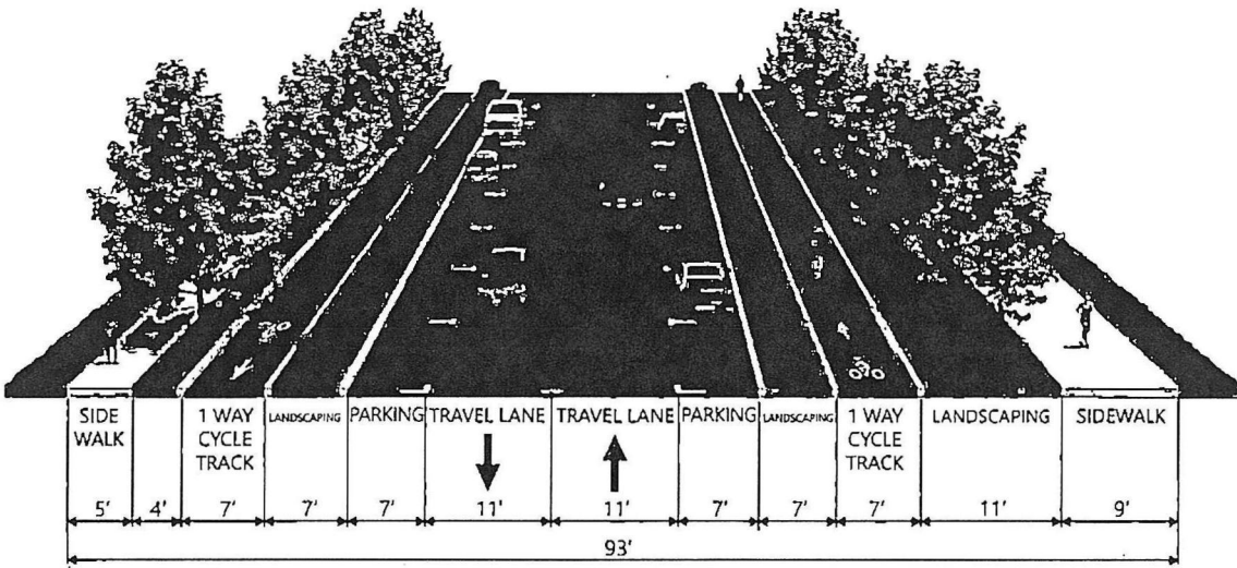
CROSS-SECTION SOUTH OF MICHELSON DRIVE
