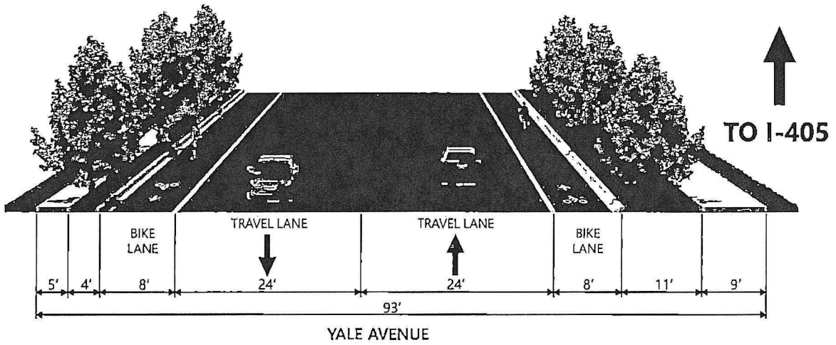
EXISTING TYPICAL CROSS-SECTION OF YALE AVENUE BETWEEN 350 FEET NORTH OF MICHELSON DRIVE AND UNIVERSITY DRIVE
