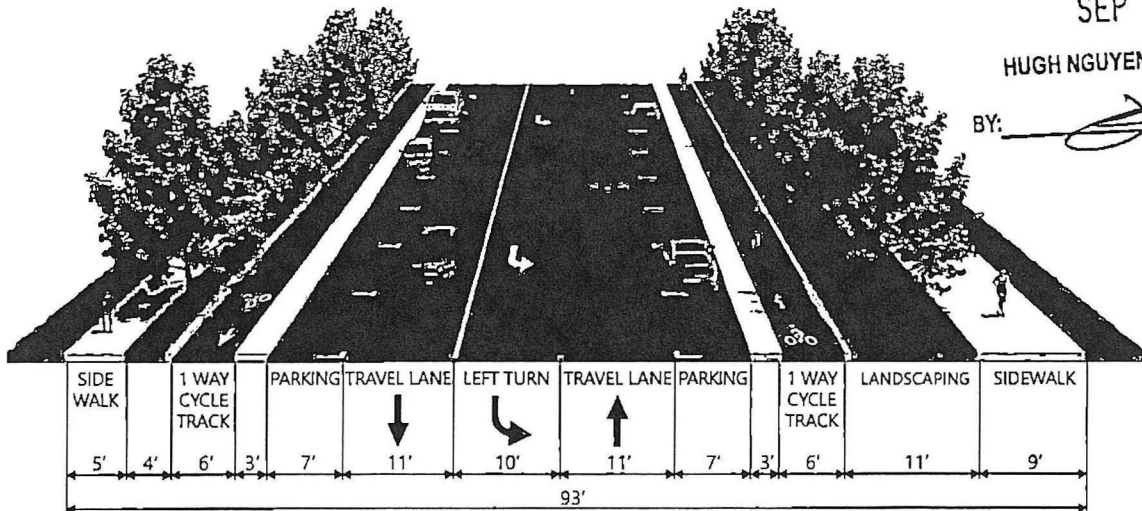
CROSS-SECTION NORTH OF MICHELSON DRIVE
