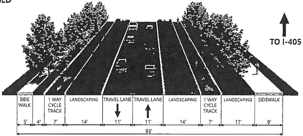
CROSS-SECTION NORTH OF UNIVERSITY DRIVE
