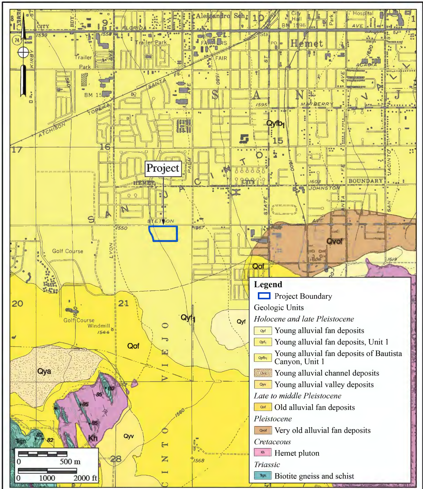
Figure 3 Geologic Map
