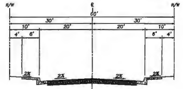
TYPICAL STREET SECTION LOCUST AVENUE N.T.S.
