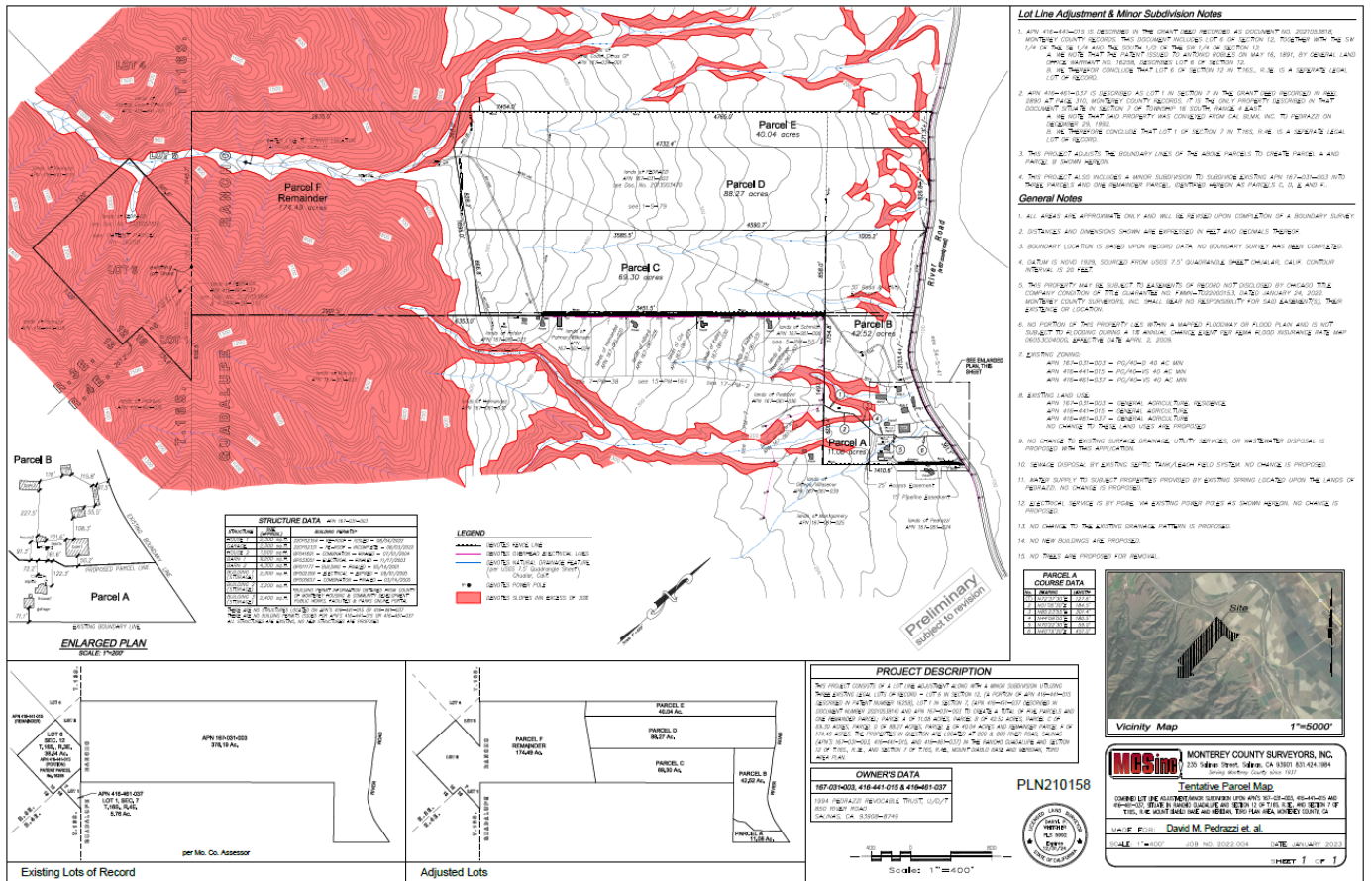
FIGURE 1 – SITE PLAN
