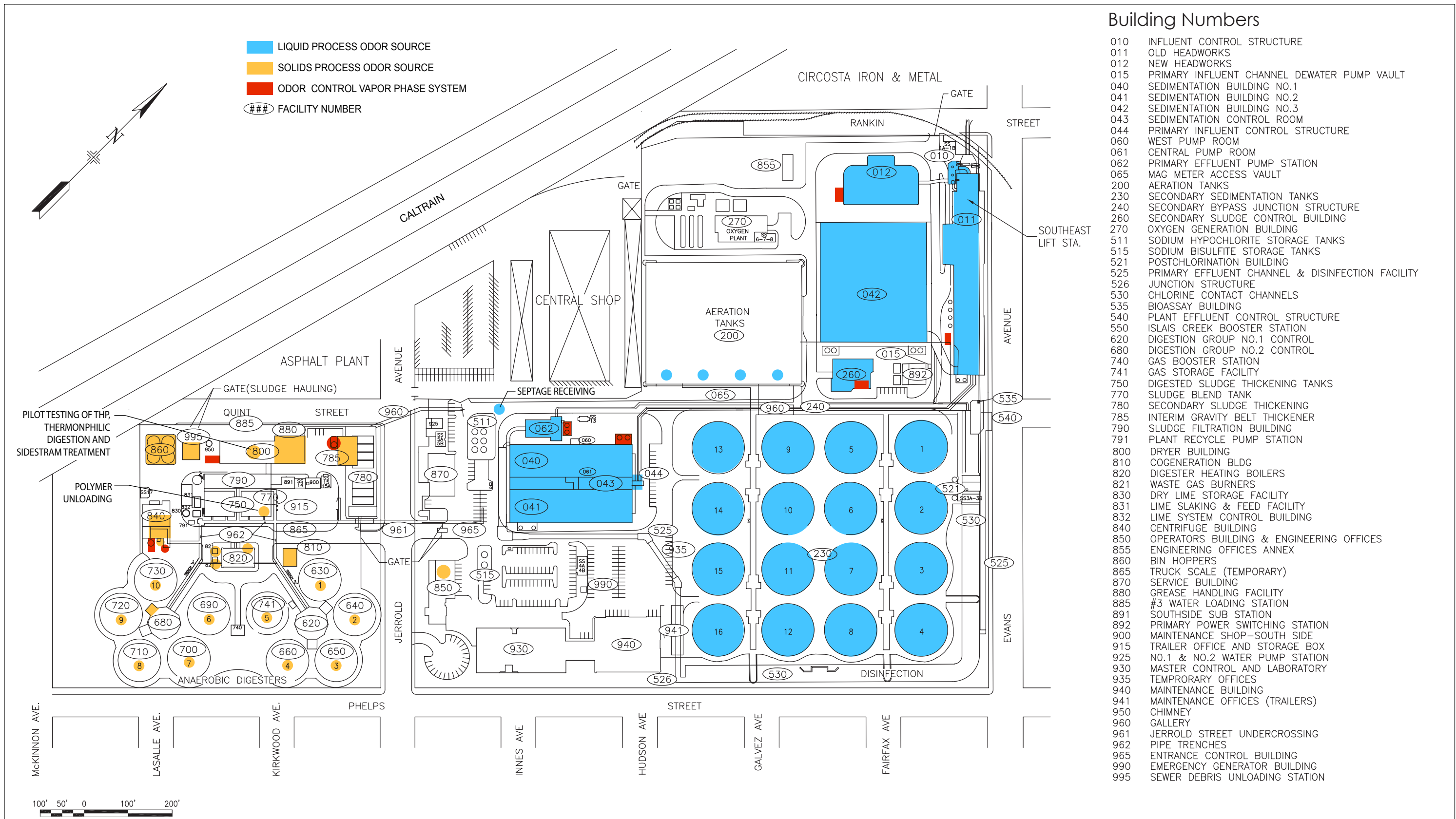
Figure 4.8-3 Existing Odor Sources and Odor Control Units at the SEP
