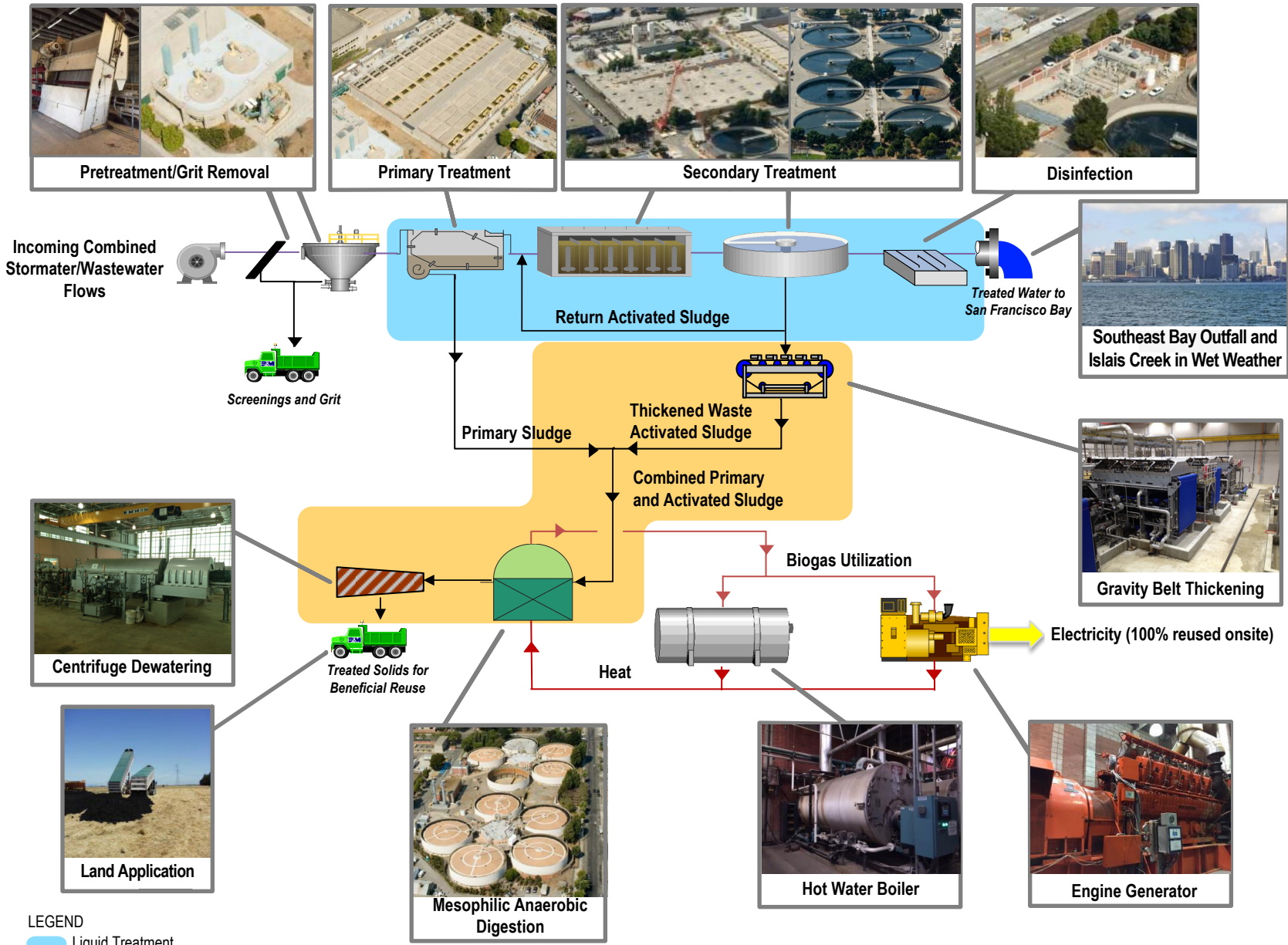
Figure 2-4 Process Flow Diagram for Existing SEP
