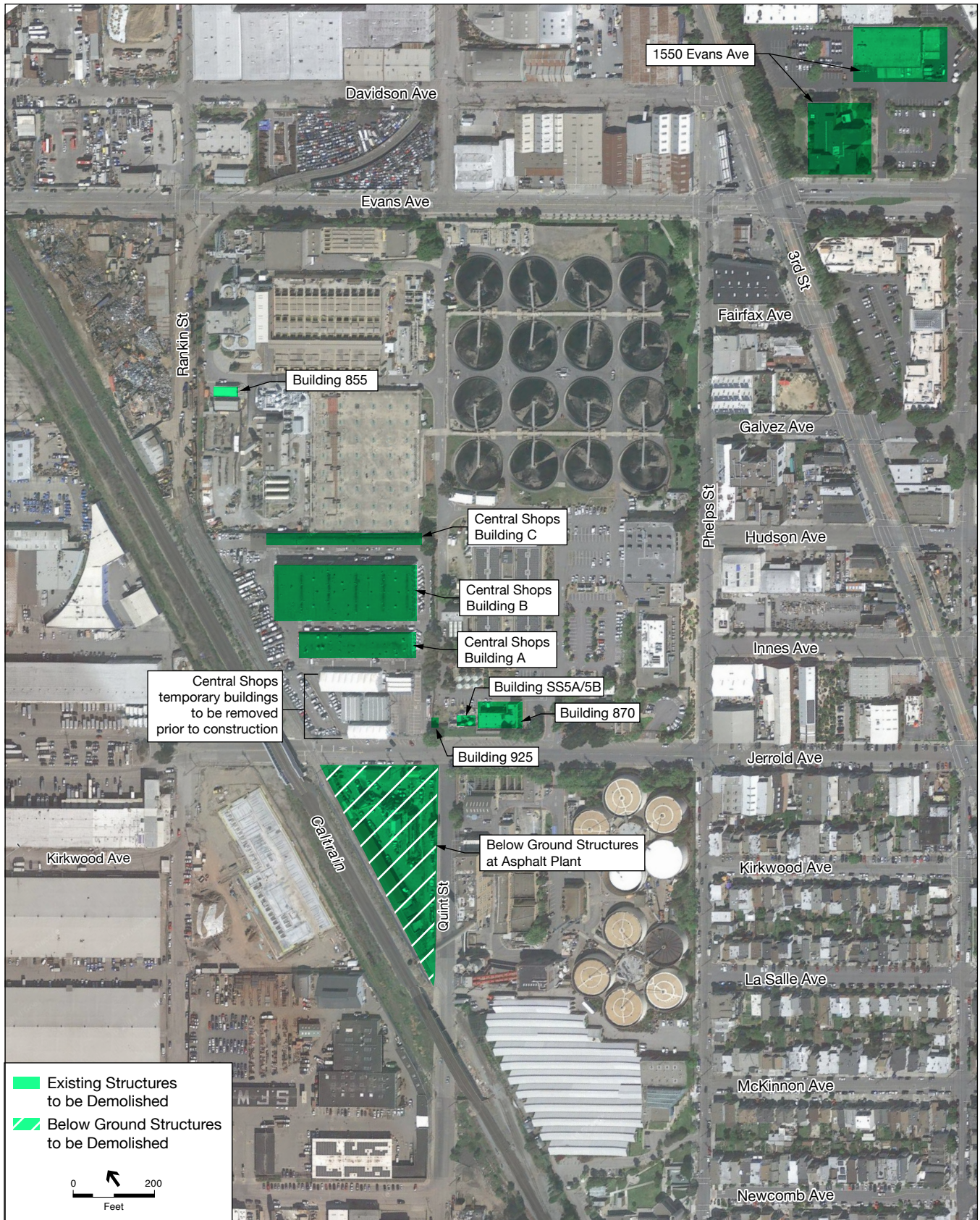
SFPUC Biosolids Digester Facilities Figure 2-17 Existing Structures to be Demolished
