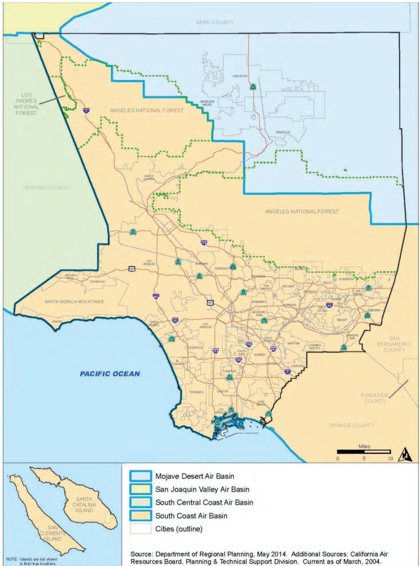
Figure 5.2-1. Air Basins
