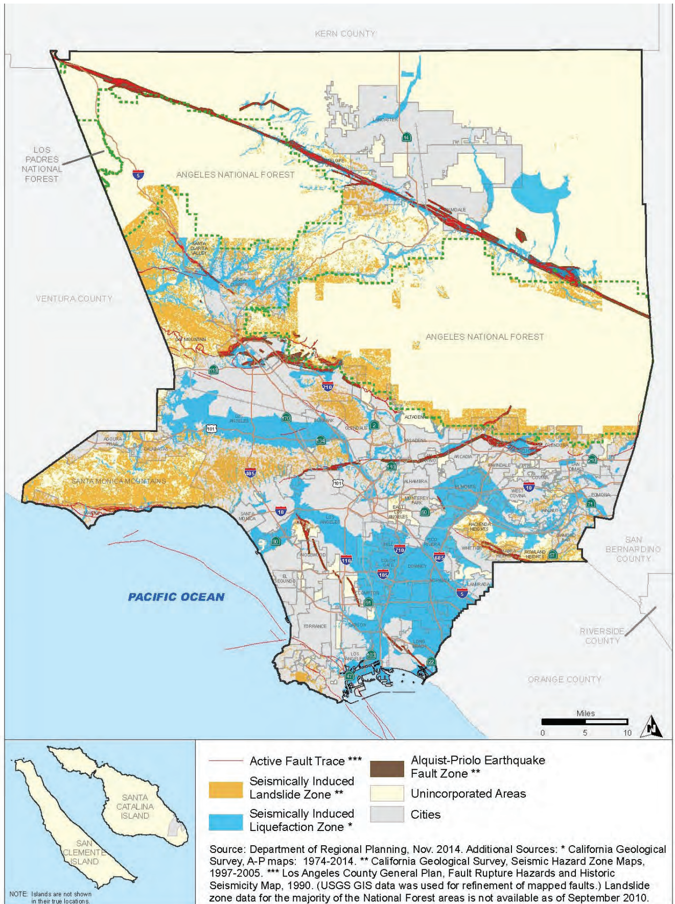
Figure 5.5-1. Seismic and Geotechnical Hazard Zones
